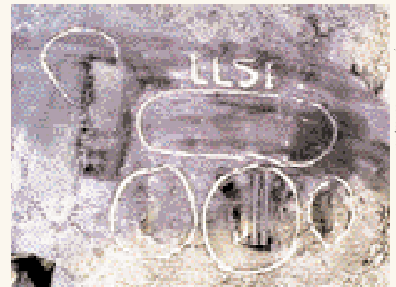
Photo 3. A widespread problem of construction damage: Bulldozer track cuts in geomembrane.
